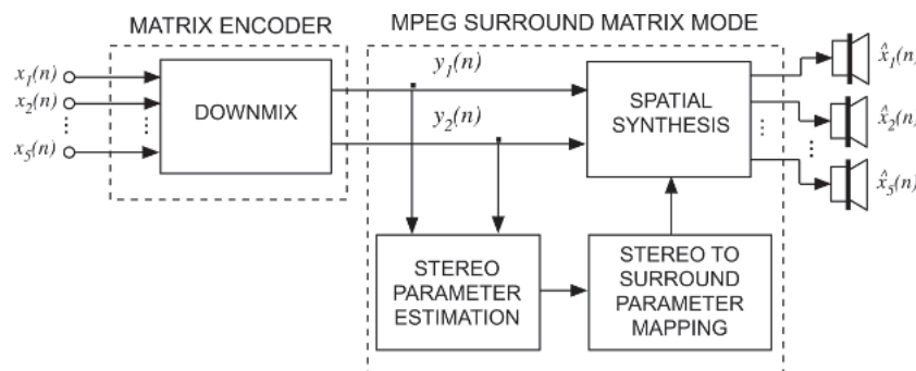
Fig. 14. MPEG Surround decoding without side information.
