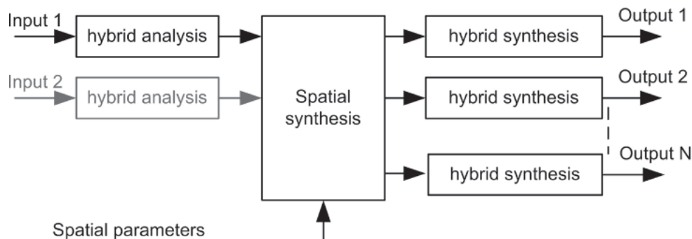
Fig. 2. High-level overview of MPEG Surround synthesis.
